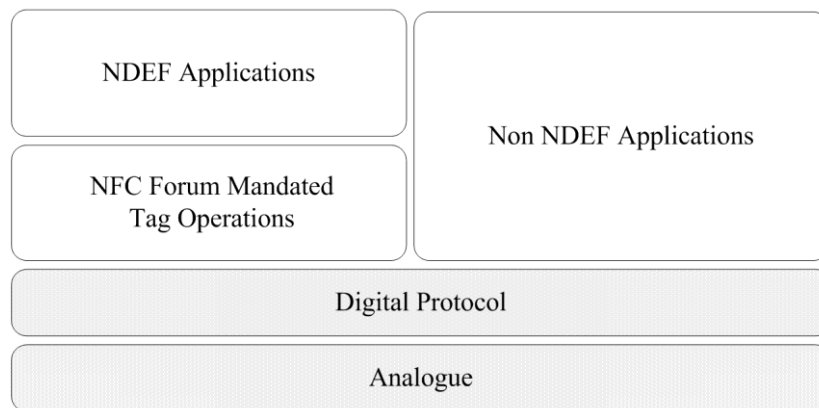
Figure 8. Protocol Stack of Reader/Writer Operating Mode
