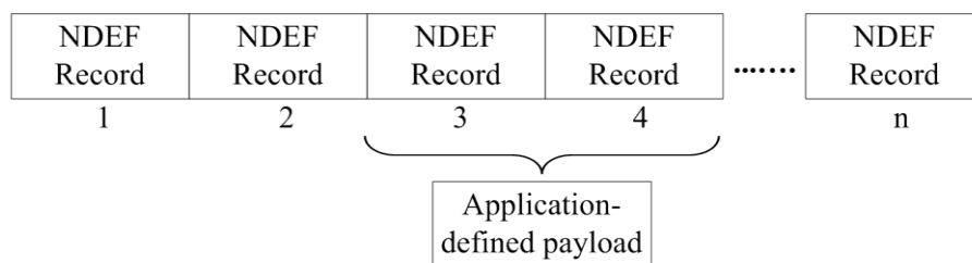
Figure 6. NDEF Message with a Set of Records
