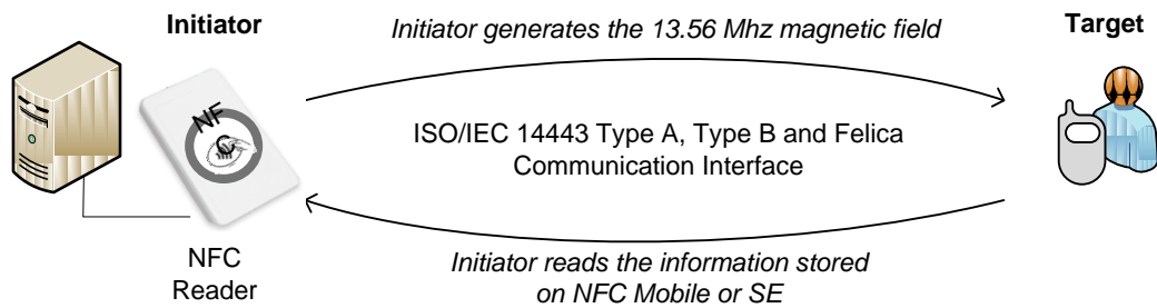
Figure 11. Card Emulation Operating Mode
