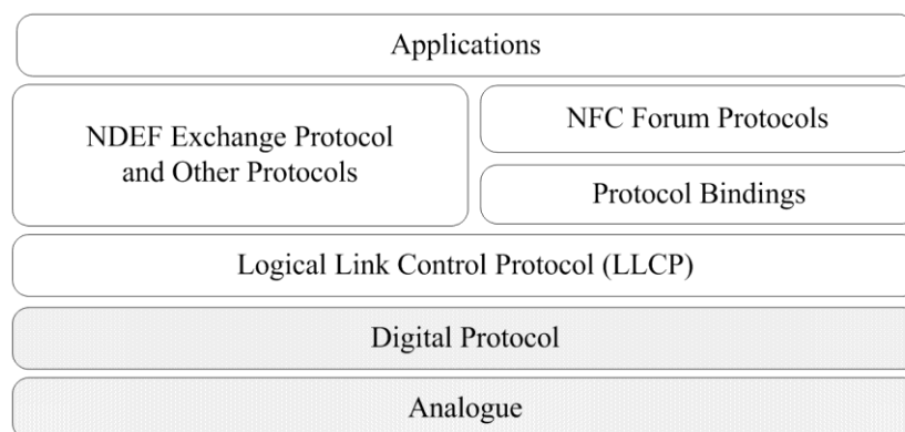
Figure 10. Protocol Stack of Peer-to-Peer Operating Mode
