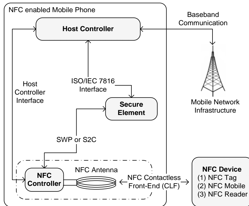
Figure 4. General Architecture of NFC enabled Mobile Phones
