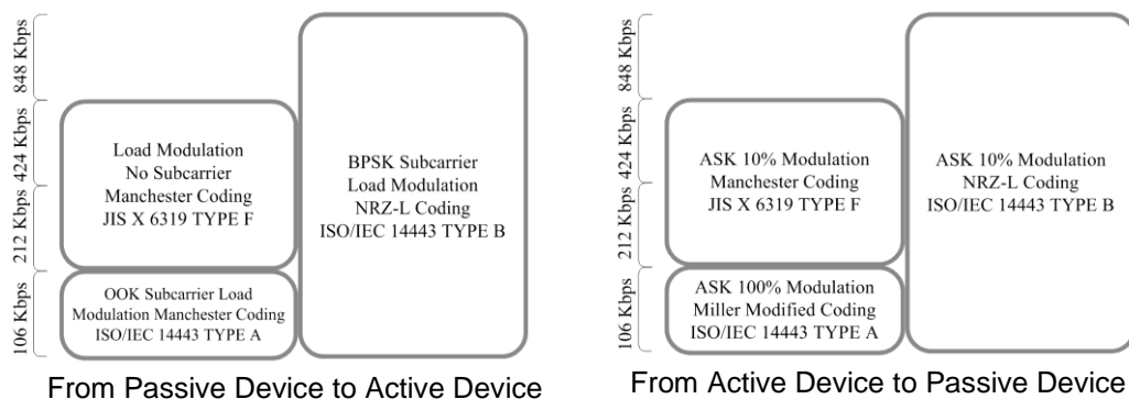
Figure 3. Modulation and Coding Schemes
